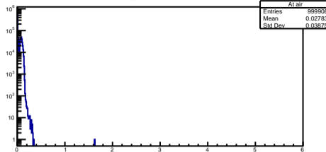
Lossed Energy in air at Alpha (d = 34mm)
