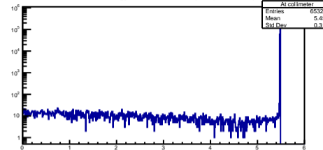
Lossed Energy in collimeter at Alpha (d = 34mm)
