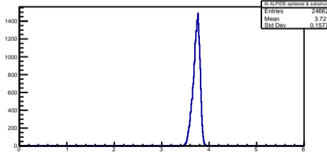
Lossed Energy in ALPIDE epitaxial + substruct at Alpha (d = 34mm)
