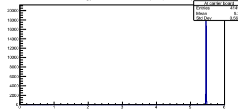
Lossed Energy in carrier board at Alpha (d = 34mm)
