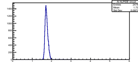
Lossed Energy in ALPIDE circuit at Alpha (d = 34mm)
